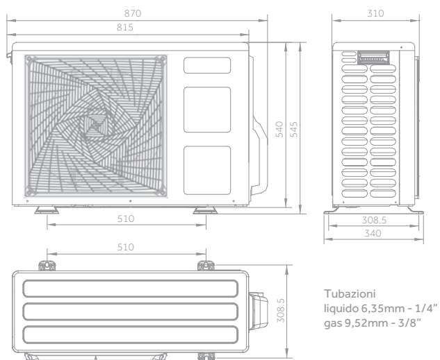
3U55S2SR2FA - 3U70S2SR2FA (3 attacchi)
